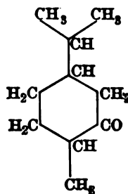
Carvomenthone.
